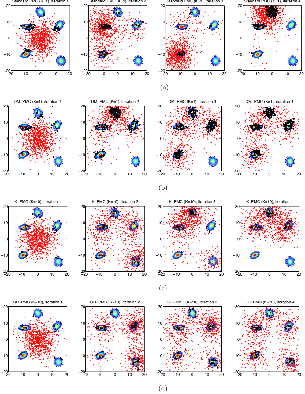
Figure A.7: ( Ex1-Section 5.2 ) Evolution of the samples before (red crosses) and after resampling (black circles) for different schemes using N = 100 and \sigma = 5 . The contour lines of the target density are also depicted. (a) Standard PMC. (b) DM-PMC ( K=1 ). (c) K-PMC ( K=10 ) with global resampling. (d) GR-PMC ( K=10 ).
